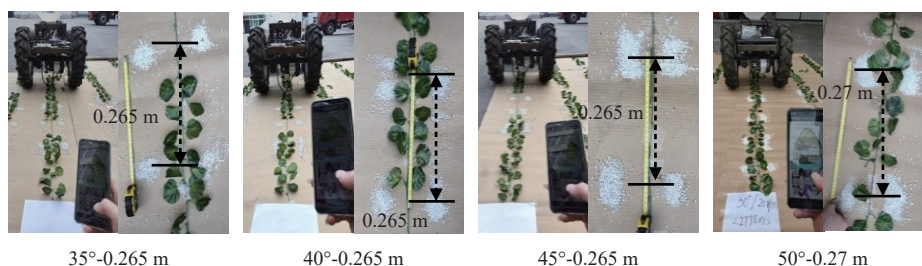
Figure 8 Test fertilization spacing under the working conditions of vehicle speed of 0.2778 m/s, rotating speed of rotating disc of 20 r/min, and fan-shaped opening of 35°-50°
